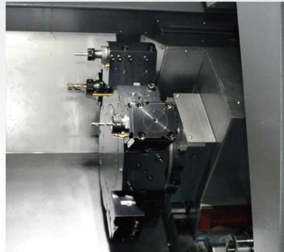
C-Axis Machining
